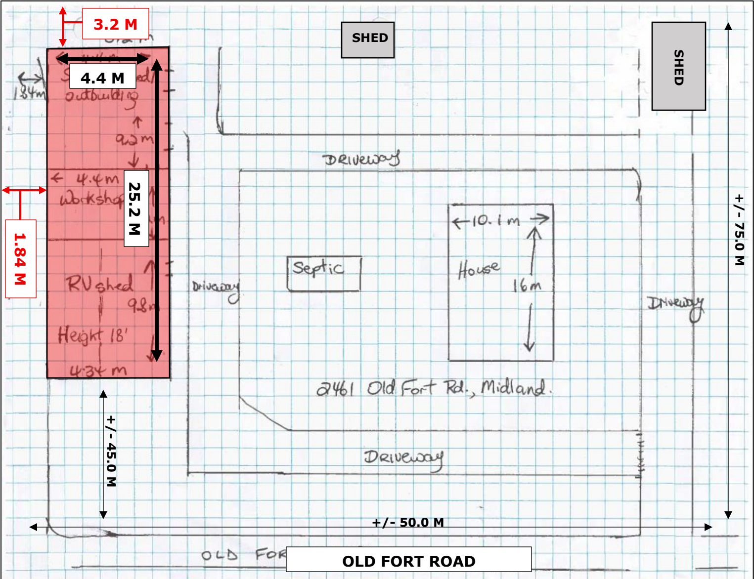
SITE PLAN
